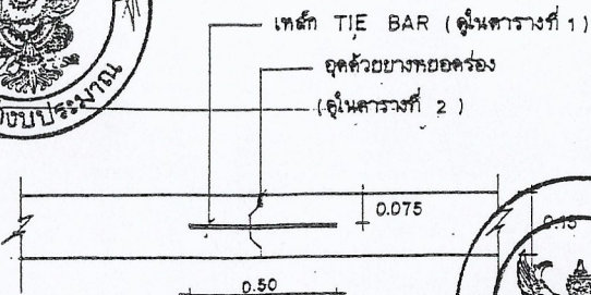
LONGITUDINAL JOINT NOT TO SCALE
